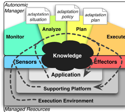
Figure 2.1: Overview of the MAPE-K autonomic control loop.
