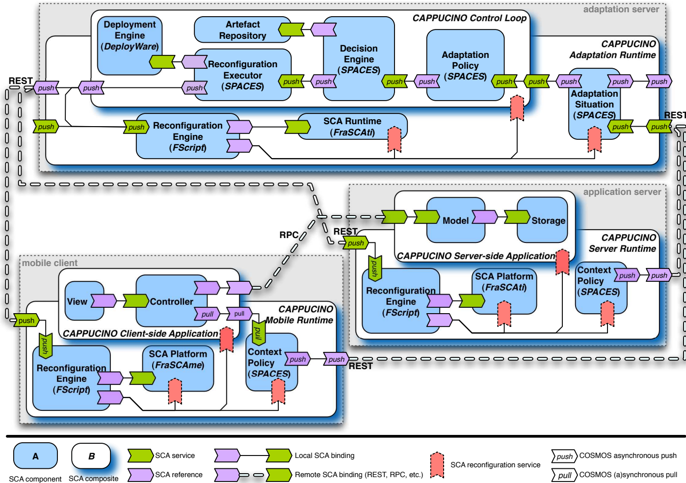
Figure 2.4: Overview of the CAPPUCINO distributed runtime.
