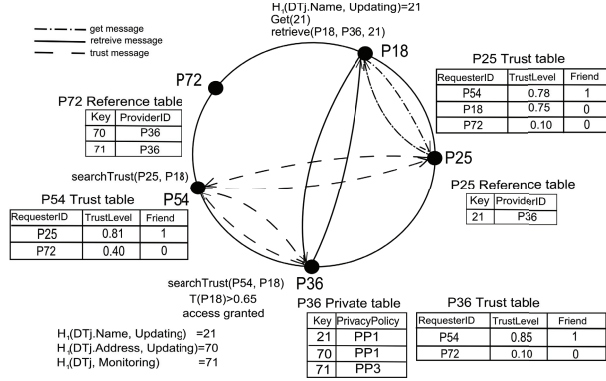
Fig. 3. Data requesting: with-friends algorithm
