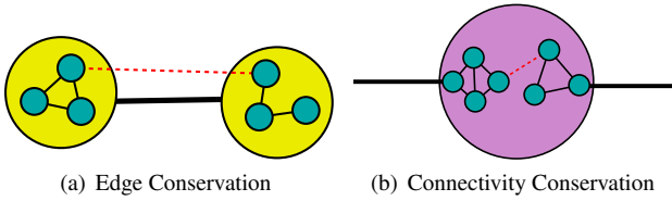
Figure 2: Edge conservation and connectivity conservation are required to preserve paths in hierarchy cuts. (a) Edge conservation ensures that edges exist between metanodes of a hierarchy cut if and only if there exists one or more edges between descendants of the metanodes. (b) Connectivity conservation ensures that paths exist through metanodes. If the red dashed edge did not exist, there would not be a path from the bold metaedge on the left through the bold metaedge on the right.
