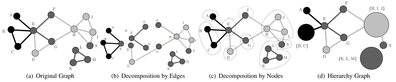
Figure 2: Steps to creating the hierarchy encoding the node and edge differences in the graph. (a) The original difference map with node and edges existing only in the first graph in black, nodes and edges existing only in the second graph in light grey, and nodes and edges existing in both graphs in dark grey. (b) Decomposition of the graph by edge difference value. The graph is divided into connected sets of edges of the same type. Nodes belonging to more than one edge set are duplicated. (c) Each connected set of edges is further clustered by node difference value. Notice the node N is clustered out of its connected edge set because it appears in both graphs whereas all the other nodes appear only in the second graph. All the nodes participating in more than one edge cluster are placed in their own cluster. (d) Final drawing of the hierarchy. Metanodes abstract the graph into clusters where every node has the same difference value and every edge has the same difference value.
