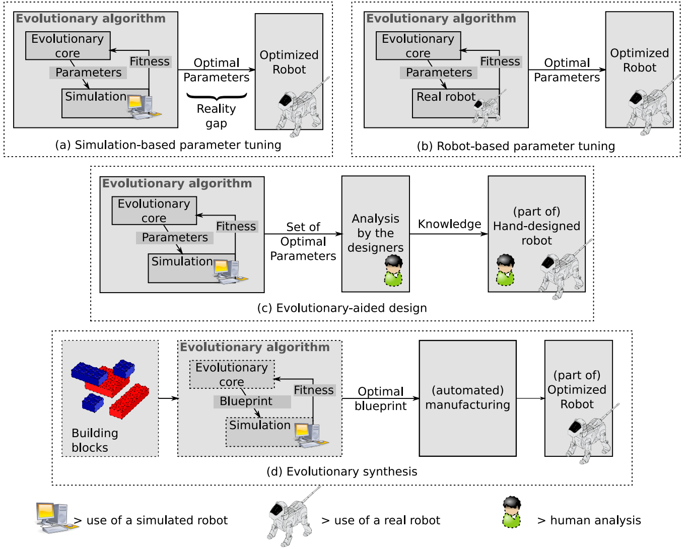
Fig. 2. Overview of the different uses of evolutionary algorithms in robotics. On this figure, “evolutionary core” denotes the basic evolutionary loop (see section II) excluding fitness evaluation. (a) Parameter tuning based on a simulation then a transfer to the real robots; (b) Parameter tuning that uses the real robot to evaluate the fitness; (c) Evolutionary-aided design (e.g. innovation); (d) Evolutionary synthesis (building blocks can be neurons, physical blocks, ...).
