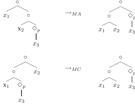
Figure 3: The structural rules of mixed associativity and mixed commutativity in flat representation and as tree rewrites
