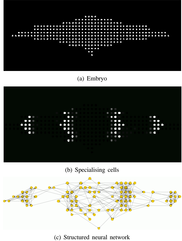
Figure 4. Development of an artificial neural network in a virtual embryo [16]. In Fig. 4(a) the embryo is depicted. white dots indicate single cells. The shape of the embryo is influencing the specialisation of cells (Fig. 4(b)) within the embryo, that later develop into nodes of the neural network (Fig. 4(c))
