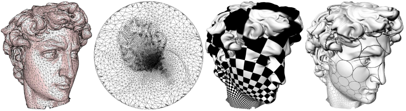
Figure 8: Conformal parameterization of the David head model over a disk-like domain. The two textures mapped onto the model illustrates the two main properties of conformal parameterization: preservation of angles and local isotropy.
