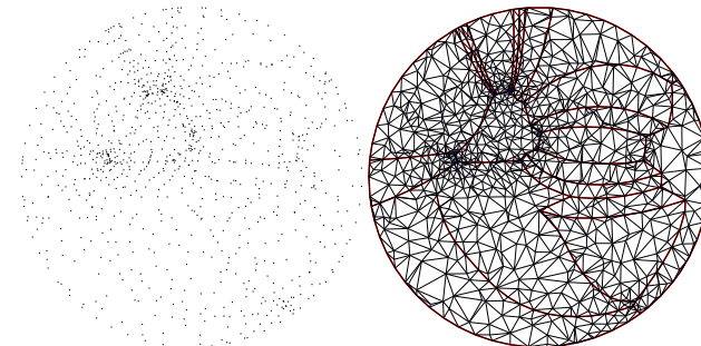
Figure 9: Constrained Delaunay triangulation.
