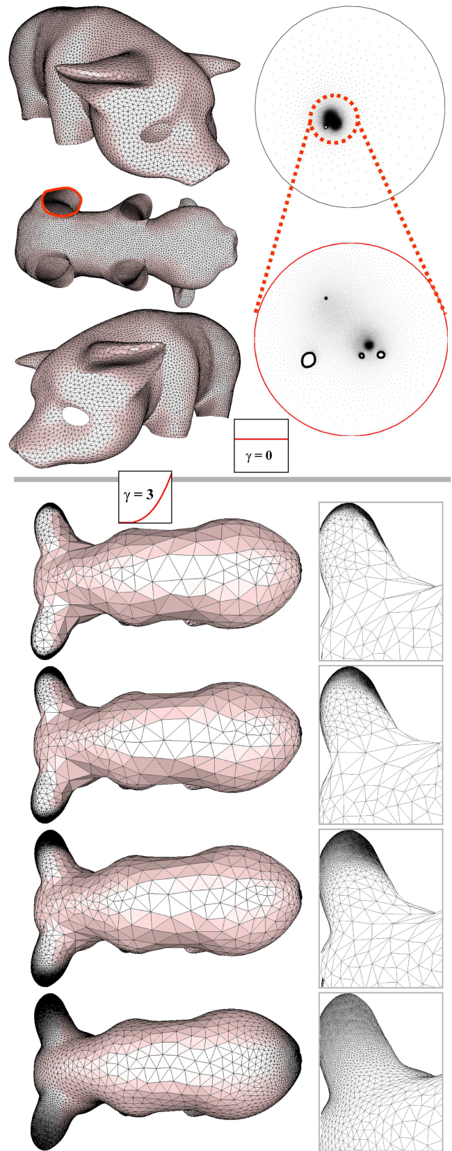
Figure 17: Top: uniform remeshing of the pig model with 15k vertices. The model has been parameterized from the longest boundary and undergoes a high range of area distortion due to flattening. Bottom: curvature-adapted remeshing with 30k vertices. The gradation is more and more smoothed by specifying 0, 3, 10 and 100 iterations for low-pass filtering the density function.
