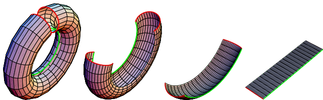
Figure 7: From an orientable surface to a polygonal schema: the torus.
