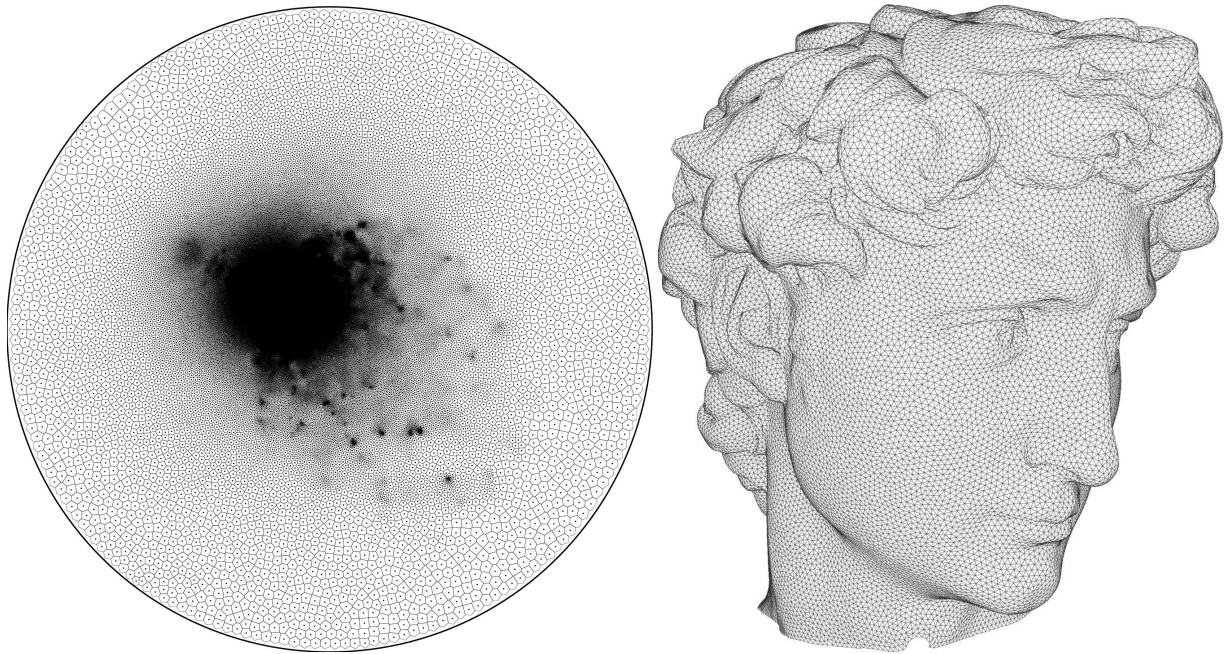
Figure 13: Weighted centroidal Voronoi tessellation built with 100 iterations of Lloyd relaxation, and final remeshing with 50k vertices
