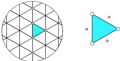
Figure 4: Uniform plane tiling with triangles.
