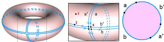
Figure 6: Left: the cut graph of the torus is composed of two pairs of twin backbones \{a; a'\} and \{b; b'\} , intentionally separated for better visualization purpose. Middle: closeup on the branching node of the cut graph. Vertices are labeled according to their multiplicity. Right: the torus has been parameterized on a disk-like domain, 4 instances of the branching node have been generated and will later be merged during the stitching.
