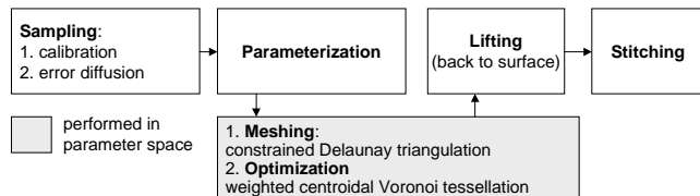
Figure 2: Remeshing pipeline.
