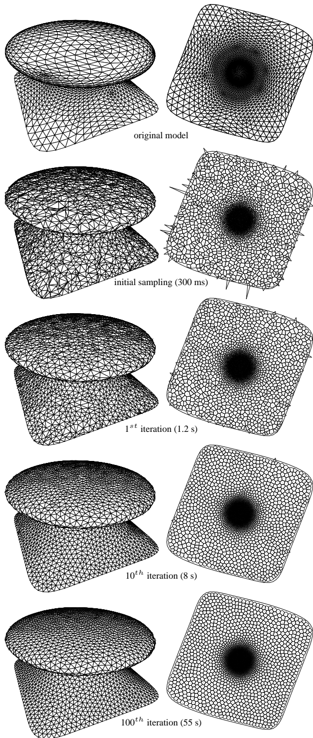
Figure 11: Top row: original mushroom model to resample and its boundary-free parameterization on a disk-like domain. Row 2: initial uniform sampling of 3k vertices generated by direct error diffusion (300 ms). Row 3: first iteration of Lloyd algorithm with a variable density coming from the area distortion due to parameterization (1.2 s). Row 4: 10 th iteration of Lloyd algorithm (8 s). Row 5: 100 th iteration of Lloyd algorithm (55 s).
