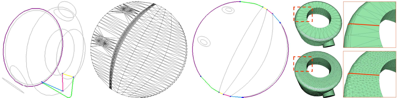
Figure 16: Uniform remeshing of the genus-1 rotor model with 10k vertices. From left to the right: cut graph (colored) and feature skeleton (light grey); mesh parameterization on a disk-like domain, and associated parameterized feature skeleton (boundary backbones with identical colors are associated pairwise). Far right, top to bottom: original, and remeshed model. Two closeups over the cut graph illustrate the univariate sampling performed along seaming backbones.
