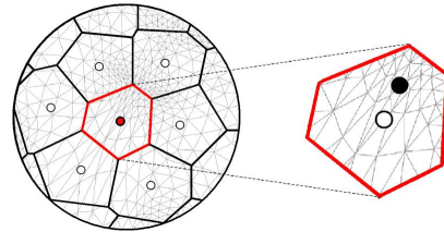
Figure 10: Left: the Voronoi cell surrounding a sample overlaps the original mesh. Right: closeup on the intersection computed between a Voronoi cell and the original mesh. The new centroid (filled) of the cell is computed as a weighted contribution of the centroids computed on the linearly interpolated polygons.
