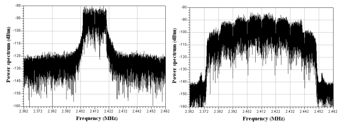
Fig. 3. Power spectral density before and after code multiplexing.
