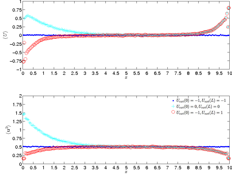
FIGURE 3. Unhomogeneous Dirichlet conditions and m = 0 . The \langle U \rangle(T, \cdot) and \langle u^2 \rangle(T, \cdot) behaviour in the confined interval [0, L] from the simulation of system (59). Three sets of boundary forcing are applied at x = 0 and x = L .
