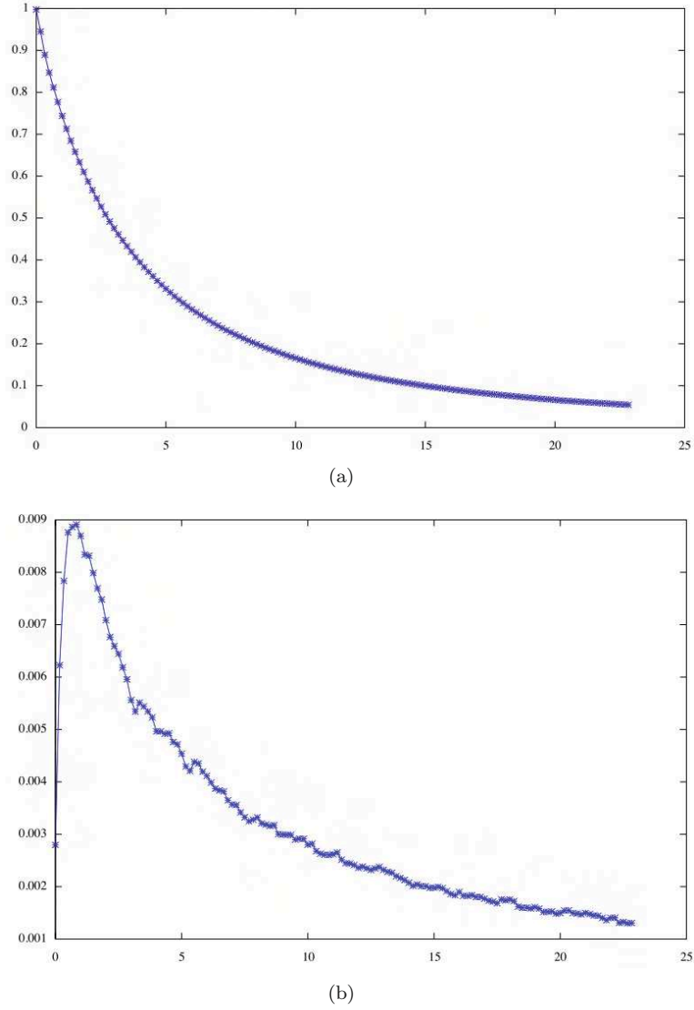
FIGURE 6. Idealized simulation of SDM with constant boundary forcing terms. (a) Time evolution of the space-averaged turbulent kinetic energy \|k\|_{L^1(\mathcal{D})} . (b) Time evolution of the L^2 norm of the zonal velocity boundary error \|U_{\text{ext}} - \langle U \rangle_{SDM}\|_{L^2(\partial\mathcal{D})} .
