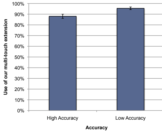
Figure 8: Probability of use of the multi-touch extension for the viewports. Error bars represent 95% confidence interval.
