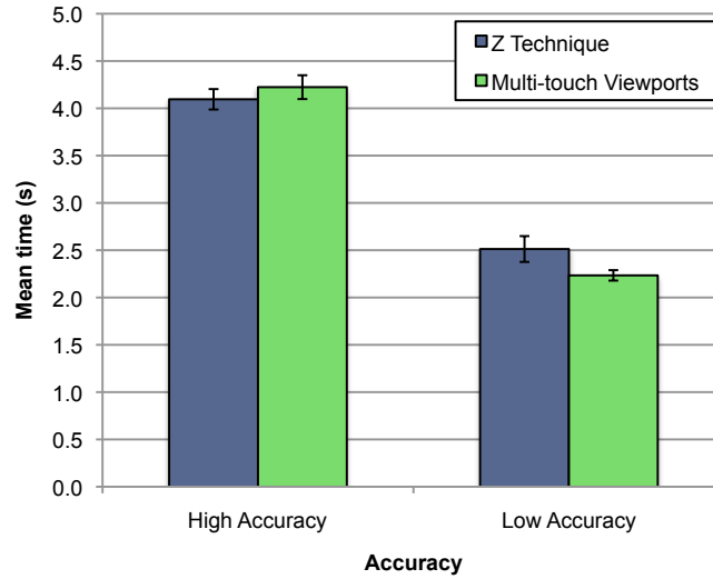
Figure 6: Mean positioning time for each technique and accuracy. Error bars represent 95% confidence interval.
