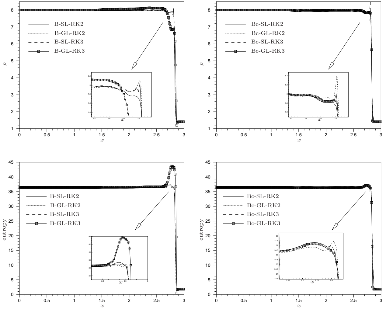
Figure 31: Double Mach reflection. Solution across the oblique shock ( y = 0.6 ). Top row : density. Bottom row : entropy. Left column : B scheme. Right column : Bc scheme.
