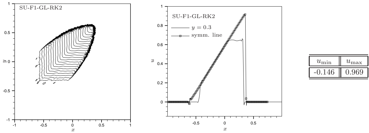
Figure 18: 2d Burger's equation : SU-F1-GL-RK2 scheme. Left : contours at time t = 1 . Middle : solution along the line y = 0.3 and along the symmetry line. Right : minimum and maximum values of the solution.
