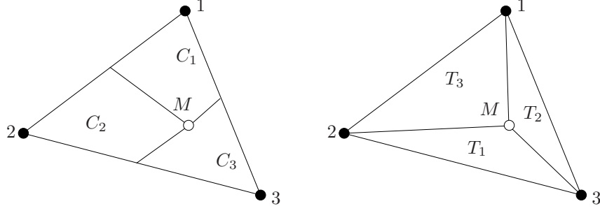
Figure 1: Left. Formulation 3 : dual areas C_j , |C_j| = \beta_j|T| . Right. Formulation 4 : area coordinates of the distribution point M ; |T|_j = \beta_j|T|
