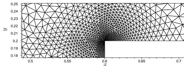
Figure 33: Mach 3 wind tunnel : close-up view of the mesh around the corner ( h = 1/80 far from the corner, h = 10^{-3} at the corner)
