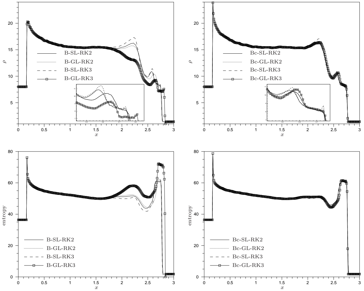
Figure 32: Double Mach reflection. Solution along the wall ( y = 0 ). Top row : density. Bottom row : entropy. Left column : B scheme. Right column : Bc scheme.
