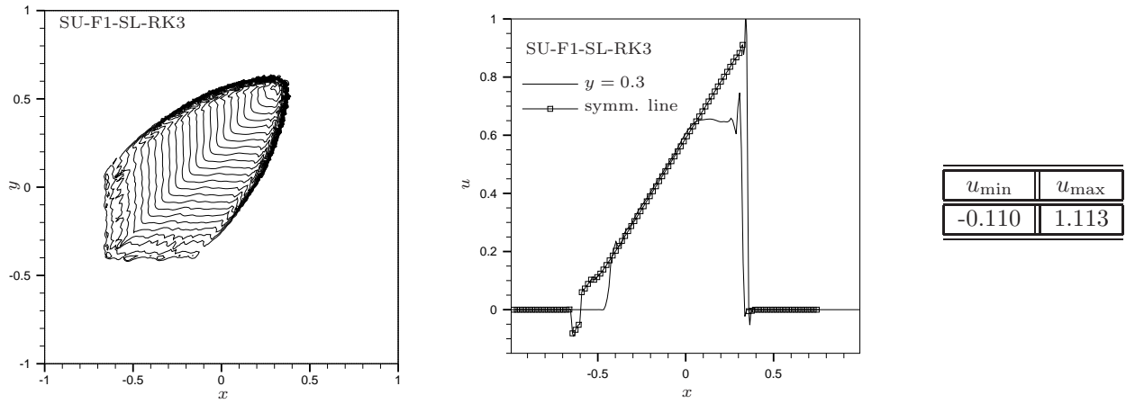
Figure 19: 2d Burger's equation : SU-F1-SL-RK3 scheme. Left : contours at time t = 1 . Middle : solution along the line y = 0.3 and along the symmetry line. Right : minimum and maximum values of the solution.
