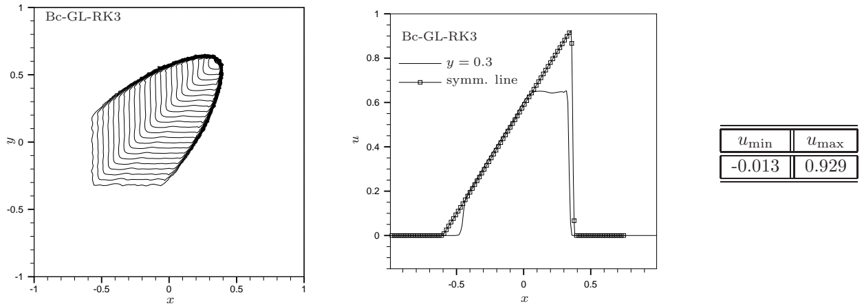
Figure 24: 2d Burger's equation : Bc-GL-RK3 scheme. Left : contours at time t = 1 . Middle : solution along the line y = 0.3 and along the symmetry line. Right : minimum and maximum values of the solution.
