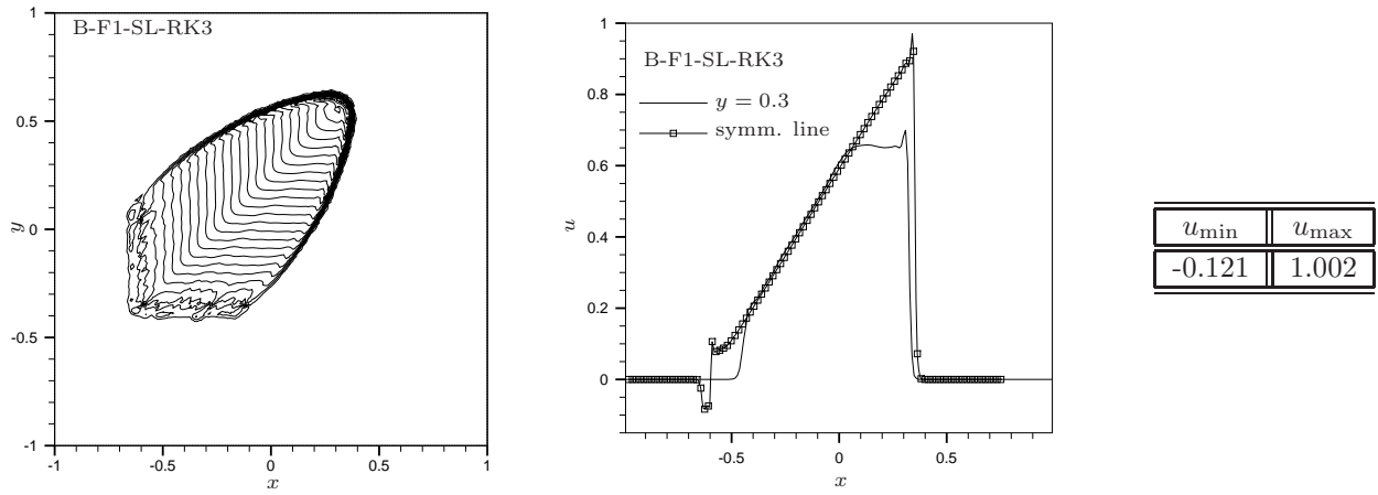
Figure 15: 2d Burger's equation : B-F1-SL-RK3 scheme. Left : contours at time t = 1 . Middle : solution along the line y = 0.3 and along the symmetry line. Right : minimum and maximum values of the solution.
