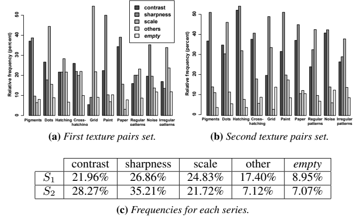
Figure 2: Relative frequency at which the criteria have been used: For each texture pair (a,b) and for each series (c).
