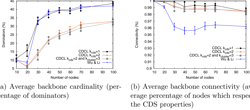
Fig. 7. Impact of the number of nodes (horizontal scalability): 5 m.s -1 , degree of 10
