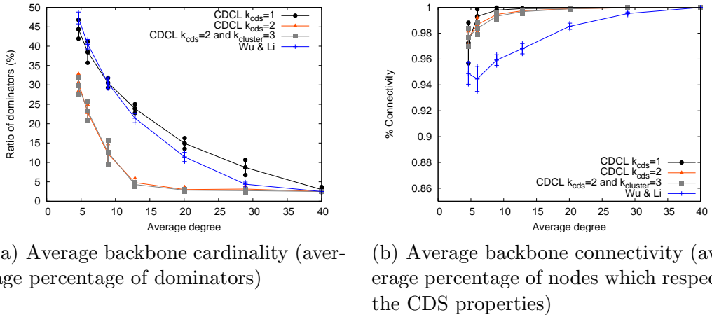
Fig. 8. Impact of the density (average number of nodes per km 2 ): 40 nodes, 5 m.s -1
