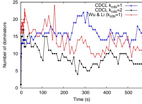
(a) Impact of the maximal distance from one dominatee to the backbone ( k_{c ds} )
