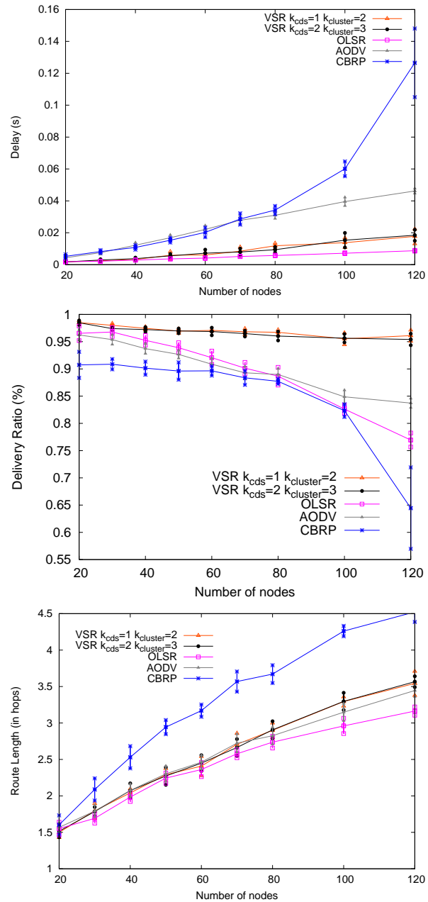
Figure 5. Horizontal scalability
