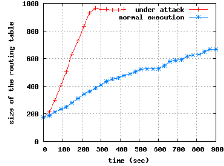
Fig. 3. Filling of the routing table under attack
