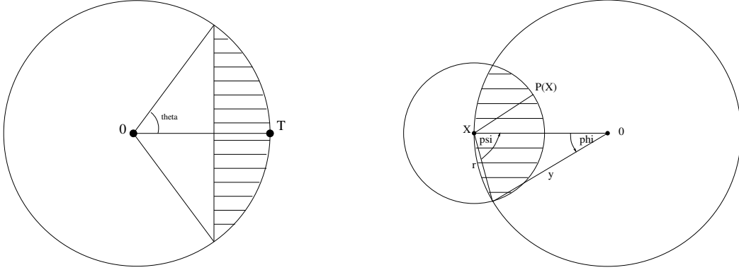
Fig. 21.3 Left : the surface of the dashed lens is equal to \frac{|T|^2}{2} |2\theta - \sin 2\theta| . Right : the dashed lens.
