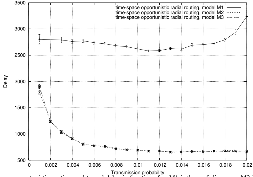
Fig. 22.6 Effect of fading on opportunistic routing: end-to-end delay in function of p . M1 is the no fading case; M2 is slow fading and M3 fast fading (both Rayleigh).
