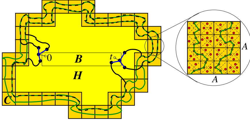
Fig. 19.1 Three disjoint paths of the Delaunay graph connecting 0 to t .
