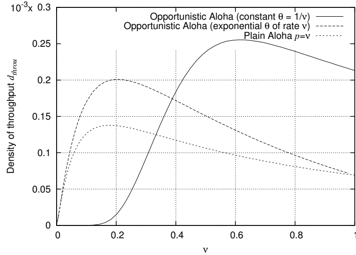
Fig. 16.5 The density of throughput of Opportunistic Aloha as a function of its parameter \nu and that of plain Aloha. Assumptions are as on Figure 16.2.
