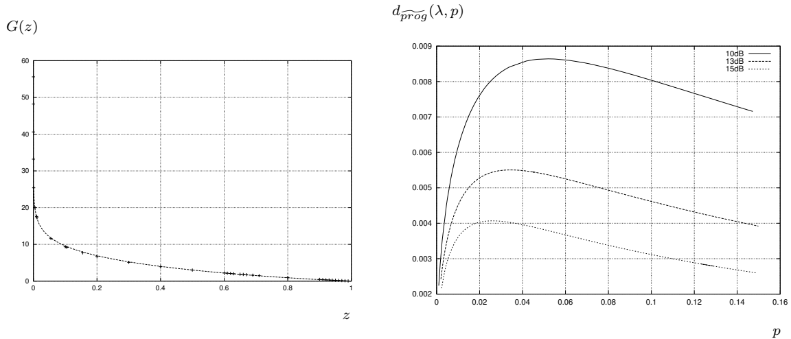
Fig. 16.6 Left: Plot of the function G_{\sim} with points representing values of G . The total relative error \frac{1}{36} \sqrt{\sum \frac{(G(z) - G_{\sim}(z))^2}{G^2(z)}} , where the summation is taken over 36 points marked on the plot, is less than 1.27%. Right: Density of modified progress d_{\text{prog}}^{\sim}(\lambda, p) for the \frac{M}{0+M/M} model with OPL 3. Here \beta = 3 , \lambda = 1 and with T = \{10, 13, 15\} dB (curves from top to bottom). The optimal values ( \arg \max, \max ) are \{(0.052, 0.0086), (0.035, 0.0055), (0.026, 0.0040)\} respectively.
