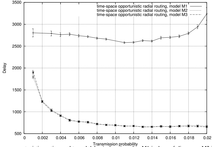
Fig. 21.6 Effect of fading on opportunistic routing: end-to-end delay in function of p . M1 is the no fading case; M2 is slow fading and M3 fast fading (both Rayleigh).
