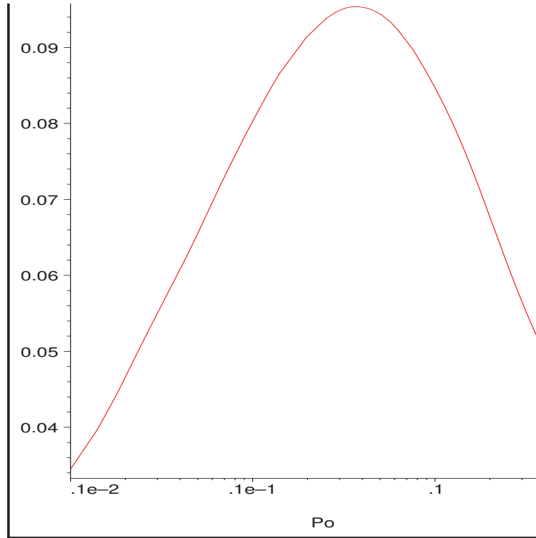
Fig. 17.2 The density of successful transmissions as defined in (17.15) for r = 1 as a function of P_o . Here \lambda = 1 , \beta = 4 , A = 1 , T = 1 , \mu = 10 .
