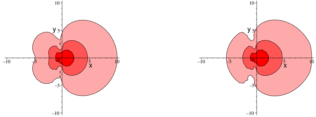
Fig. 22.2 Equal-strength power sets (path-loss level sets) for (c) with omnidirectional attenuation OPL 2 with A = 1000, \beta = 3 , and radiation patterns RP1 (left), RP2; \theta_1 = \frac{1}{12}\pi, \theta_2 = \frac{2}{3}\pi (right). The contours represent the levels t = \{100, 110, 120\} dB.
