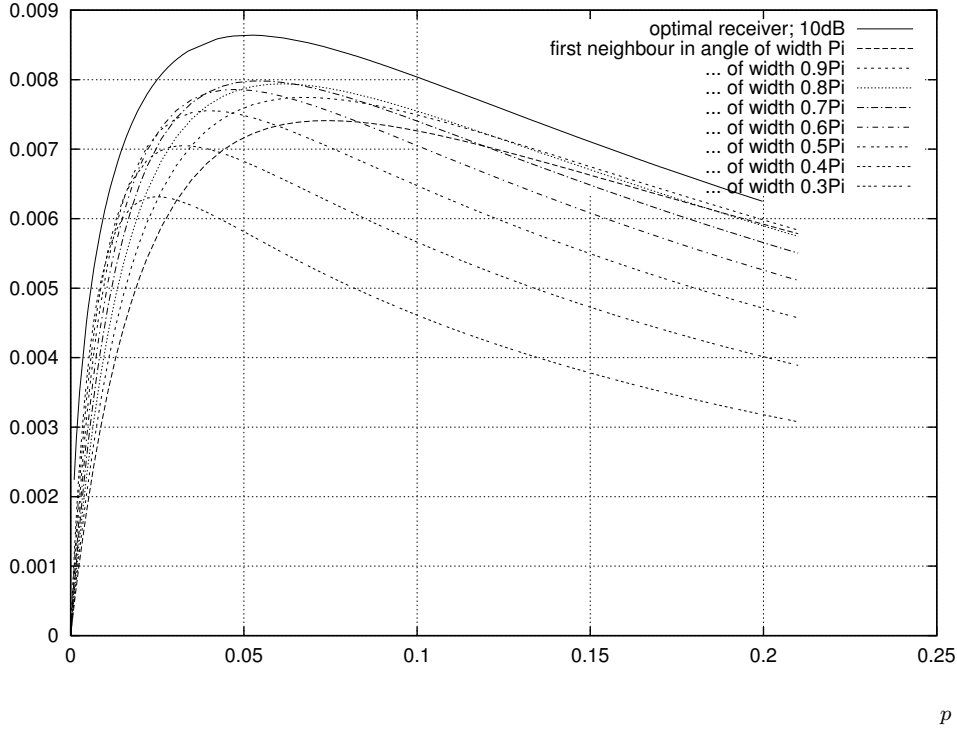
Fig. 16.7 Density of directional progress for the \frac{M}{0+M/M} model with OPL 3 with \beta = 3 , \lambda = 1 , with T = 10\text{dB} . Comparison of the opportunistic and the “smallest hop in a cone” cases.
