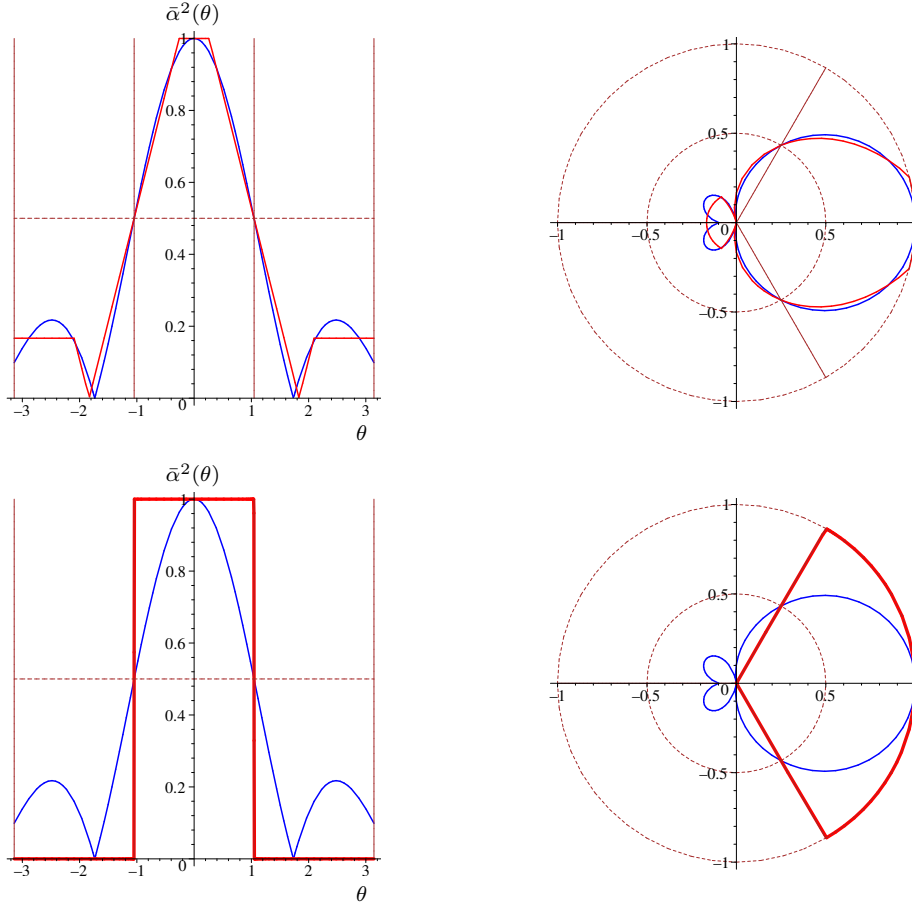
Fig. 22.1 Top: approximation of RP1 by RP2 with \theta_1 = \frac{1}{12}\pi, \theta_2 = \frac{2}{3}\pi ; Cartesian and polar plots. Bottom: in boldface/red, perfect RP modeled by RP2 with \theta_1 \rightarrow \pi/3- and \theta_2 \rightarrow \pi/3+ ; Cartesian and polar plots.
