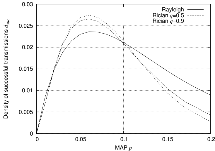
Fig. 16.3 Density of successful transmissions d_{suc} for plain Aloha in function of p in the Rayleigh and the Rician (with q = 1/2 and q = .9 ) fading cases; \lambda = r = 1 , W = 0 , and T = 10\text{dB} , \beta = 4 .
