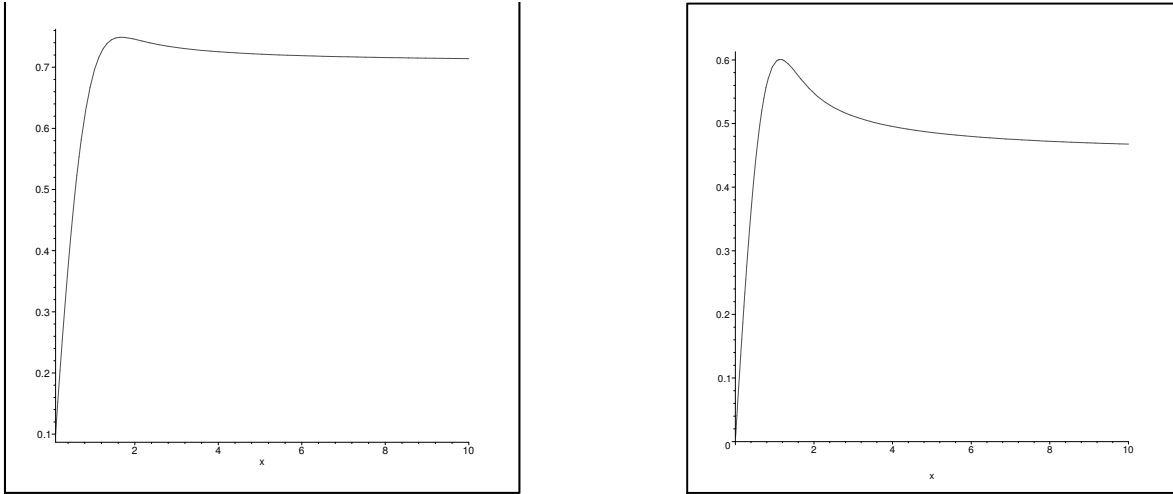
Fig. 20.4 Left: Mean of L(X) in function of x . Right: Mean of P(X) in function of x = |X| .
