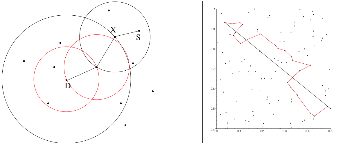
Fig. 20.1 Left: the next hop from point X on the route from S to D . Right: in red, the near-neighbor greedy route on a Poisson point process; in black, the straight line between the source and the destination, located in (.5,.5) .
