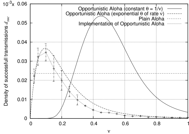
Fig. 16.2 The density of successful transmissions d_{suc} of Opportunistic Aloha for various choices of \theta . The propagation model is (16.1). We assume Rayleigh fading with mean 1 and W = 0 , \lambda = 0.001 , T = 10\text{dB} , r = \sqrt{1/\lambda} and \beta = 4 . For comparison the constant value \lambda_{\max} p_c(r, \lambda_{\max}) of plain Aloha is plotted.
