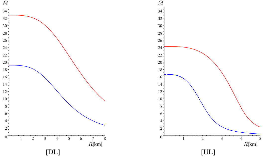
Fig. 18.1 Mean-load estimations for the downlink (DL) and uplink (UL), for the Hex model (upper curves) and PV model (lower curves). The numerical assumptions are: \alpha = 0.4 , \xi_{\downarrow} = \xi_{\uparrow} = -16\text{dB} , W^u = -105\text{dBm} , W_m = -103\text{dBm} , \tilde{P}^u = 52\text{dBm} , Q = 42.73\text{dBm} (these values correspond to the UMTS system) and \beta = 3.38 , A = 8667 yielding \bar{g}_{\text{PV}} = 1.5325 , \bar{g}_{\text{Hex}} = 0.3717 , \bar{g}_{\text{Hex}|2\beta} = 0.2283 , \bar{f}_{\text{PV}} = 1.4493 , \bar{f}_{\text{Hex}} = 0.6564 , \bar{f}_{\text{Hex}}^2 = 0.8703 , \bar{l}_{\text{Hex}} = 0.4394
