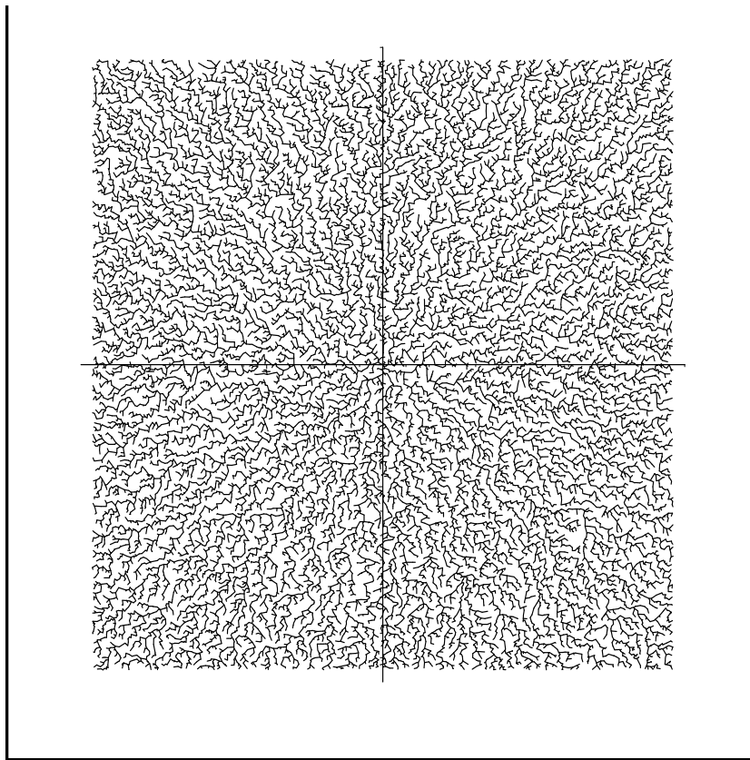
Fig. 20.2 Radial spanning tree of a Poisson p.p. in the unit square. The routing is 'smallest hop' and the graph is the complete one.
