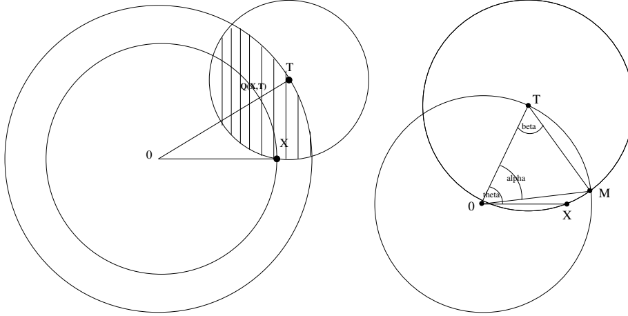
Fig. 20.5 Left : Q(r, \rho, \theta) . Right : The \alpha and \beta angles.
