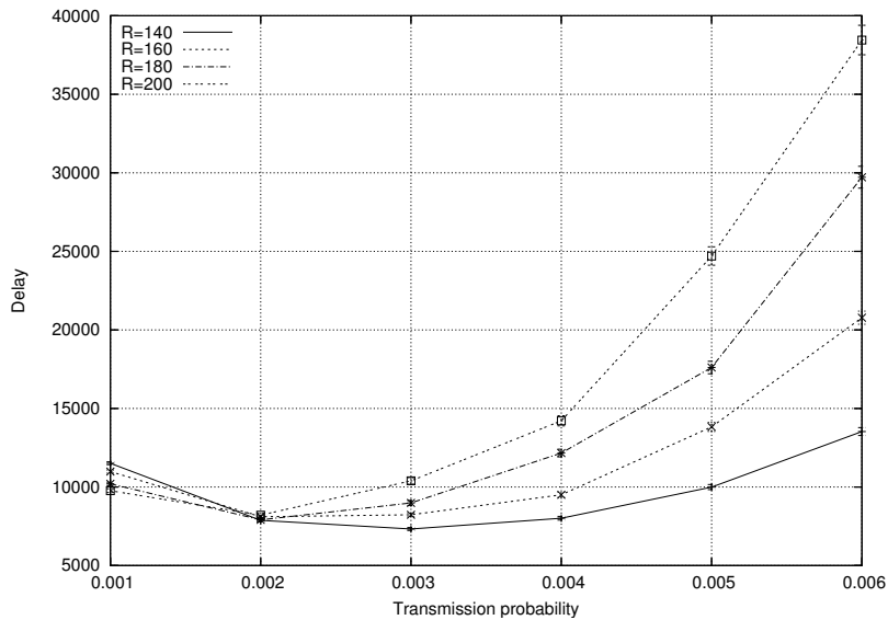
Fig. 21.4 Layer-Aware MWR: end-to-end delay versus p for various transmission ranges.
