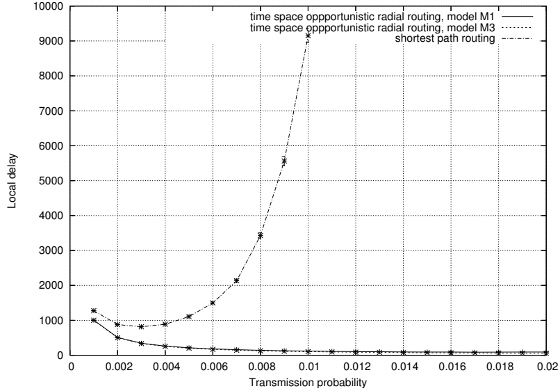
Fig. 21.8 Mean local delay for opportunistic radial routing (with and without fading) and for the layer-aware MWR algorithm.
