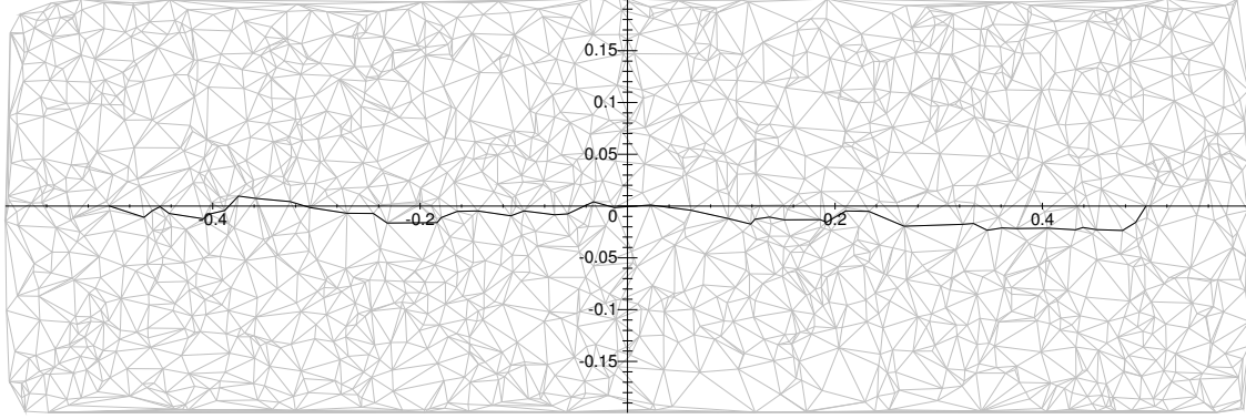
Fig. 19.2 Euclidean shortest path routing on the Poisson–Delaunay graph.
