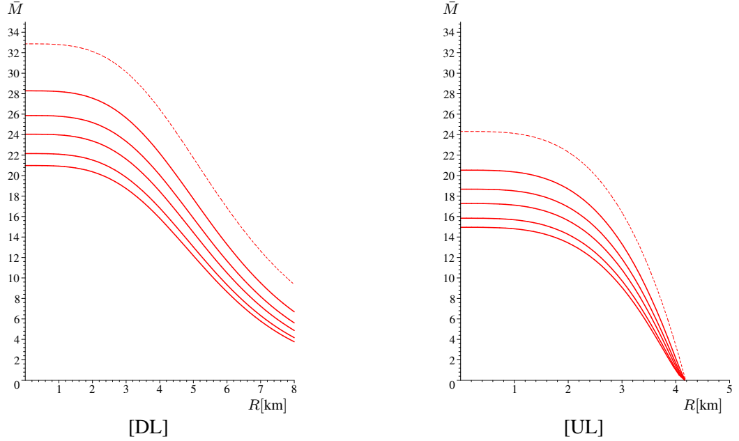
Fig. 18.2 Maximal load estimations in Honeycomb model at a given CPR \epsilon = 0.2, 0.1, 0.05, 0.02, 0.01 (solid lines) for the downlink (DL) and uplink (UL). The dashed curves represent the values for the mean model. The numerical assumptions are as on Figure 18.1. User maximal power constraints are taken into account on UL as proposed in (Baccelli, Błaszczyszyn, and Karray 2004).
