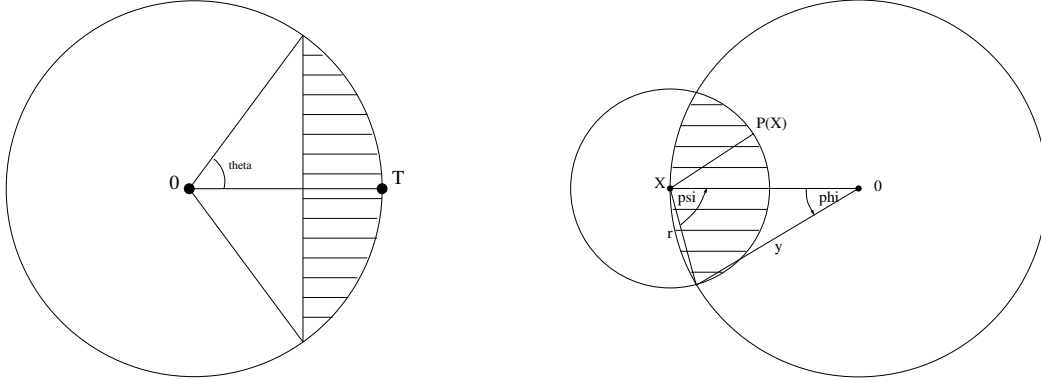
Fig. 20.3 Left : the surface of the dashed lens is equal to \frac{|T|^2}{2} |\theta - \sin 2\theta| . Right : the dashed lens.
