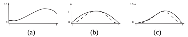
Figure 6: (a) One example of shape(x) . (b) Parabola attenuation function (plain line) and Wyvill attenuation function (dashed line). (c) Resulting weights before normalization, for each attenuation function presented. Note the non zero tangent of the weights curve obtained with the use of the parabola (plain).
