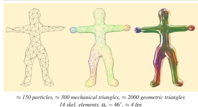
Figure 10: Skeleton-based examples, with a \frac{1}{\sqrt{r}} -like field function. The first column shows the mechanical mesh, the second is the geometric mesh and the last is a textured rendering.
