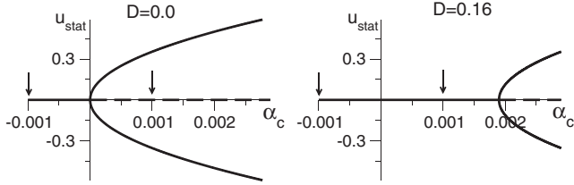
FIG. 3. Bifurcation diagram of the stationary amplitude u_c = u_{\text{stat}} subjected to the control parameter \alpha_c = \epsilon for two noise variances D . The vertical arrows denote the values of \alpha_c = \epsilon examined in Fig. 2.
