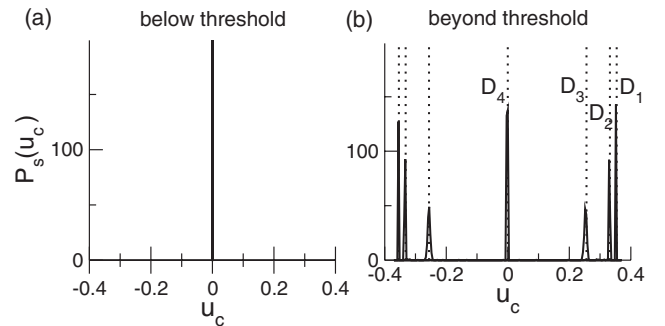
FIG. 2. The stationary probability density P_s(u_c) computed numerically for various values of \varepsilon and D and their comparison to analytical results. (a) \varepsilon = -0.001 , and the system is stable for all D . (b) \varepsilon = 0.001 and the system exhibits a single mode with \alpha_c > 0 . The different probability density functions are computed for D_1 = 0 , D_2 = 0.01 , D_3 = 0.04 , and D_4 = 0.16 and the dotted lines represent the analytical results u_{stat} = \pm(\alpha_c - \alpha_{th})/2\mu . We applied the stochastic Euler forward algorithm with dt = 0.01 for the amplitudes u_c(t) and u_0 and computed P_s(u_c) by an ensemble average over 1000 paths after 6 \times 10^5 time steps.
