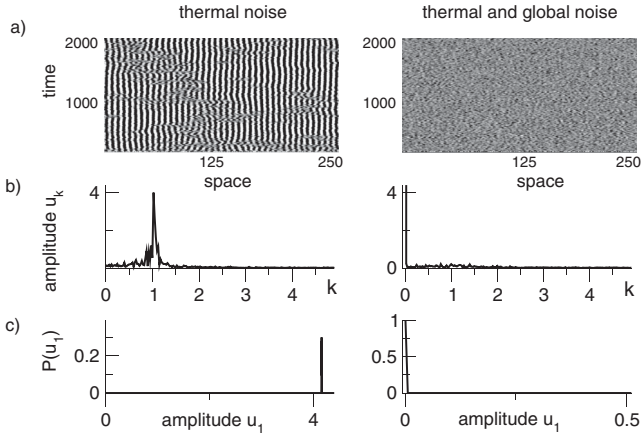
FIG. 4. Effects of global fluctuations in the presence of thermal noise. In (a), the spatiotemporal activity subtracted by its spatial average at each time is shown for thermal noise alone (left panel, D_{\text{th}} = 2.5 \times 10^{-5} , D' = 0 ) and for the sum of thermal and strong global fluctuations (right panel, D_{\text{th}} = 2.5 \times 10^{-5} , D' = 0.25 ). (b) shows the stationary probability density P(u_c) of the critical Fourier amplitudes u_c computed in the time interval t \in [35000; 35100] for both noise variances. The same numerical methods and parameters as in Fig. 1 were used.
