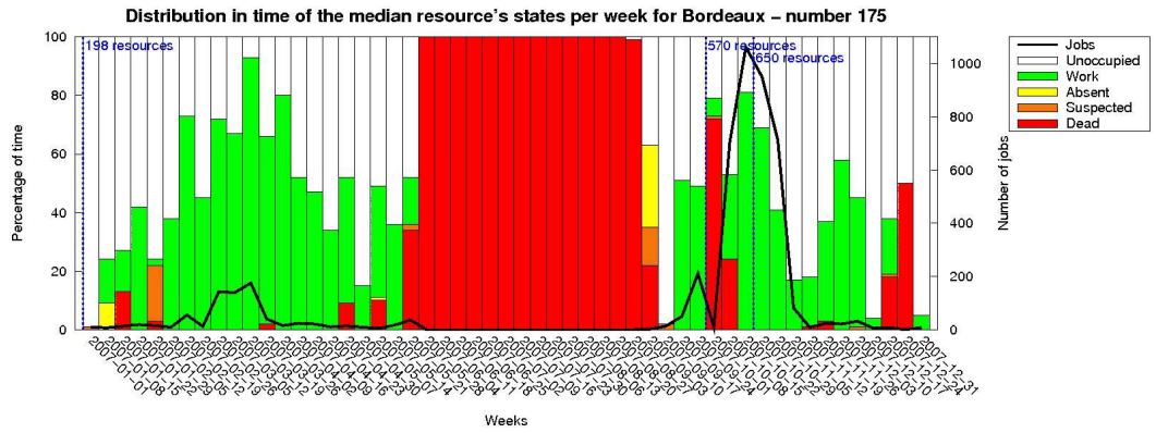
Figure 5: Median resource diagram for Grid'5000's Bordeaux site
