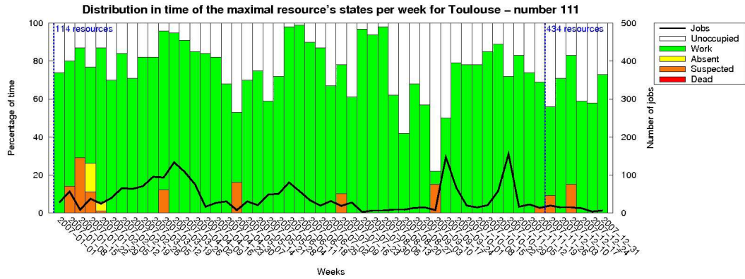
Figure 34: Maximal resource diagram for Grid'5000's Toulouse site
