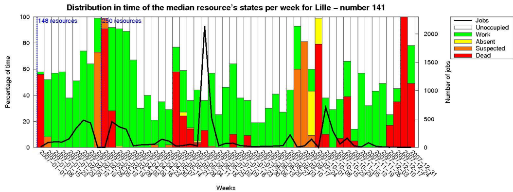
Figure 9: Median resource diagram for Grid'5000's Lille site
