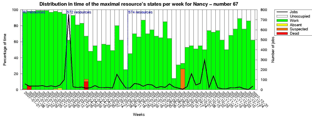
Figure 18: Maximal resource diagram for Grid'5000's Nancy site
