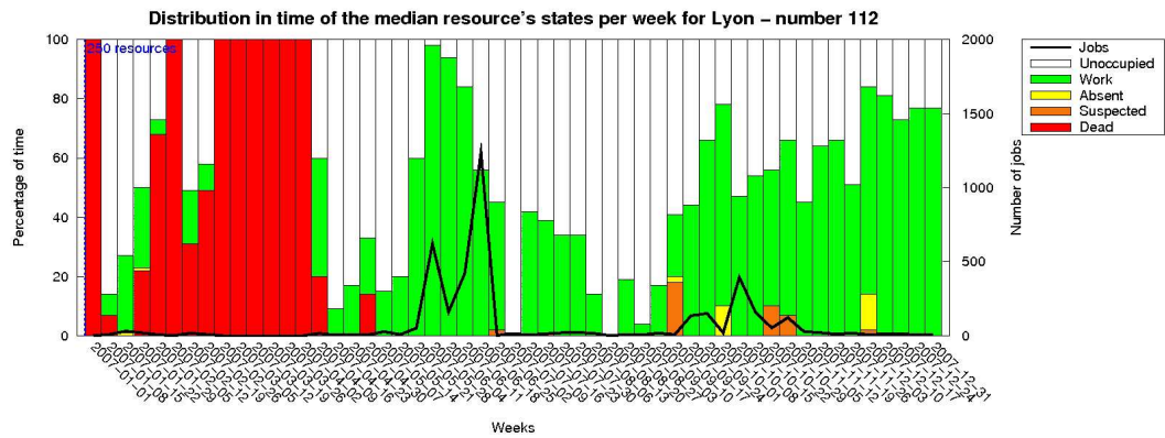
Figure 13: Median resource diagram for Grid'5000's Lyon site
