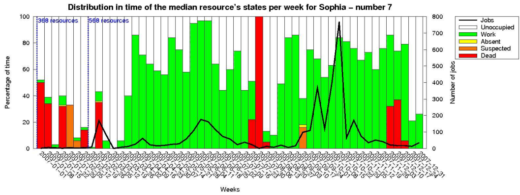
Figure 29: Median resource diagram for Grid'5000's Sophia site
