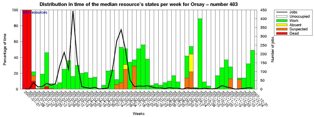
Figure 21: Median resource diagram for Grid'5000's Orsay site
