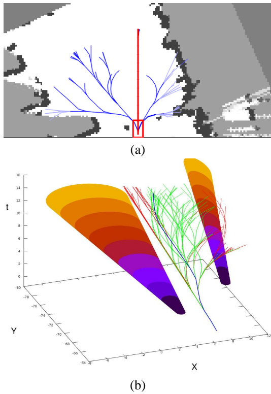
Fig. 6. (a) The RRT grow in a static occupancy grid: lighter blue is for lower likelihood. (b) The prediction of the moving obstacles and the explored tree in (x, y, t) space.
