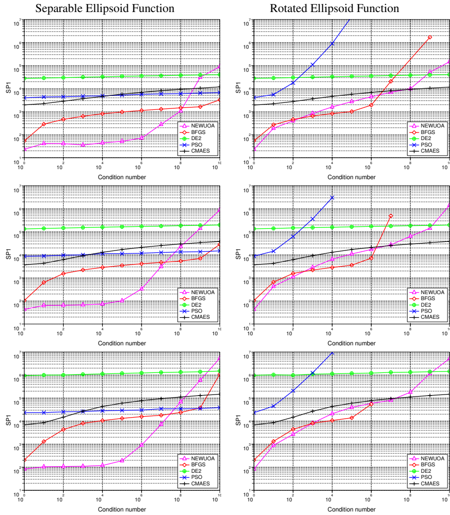
Fig. 3. Ellipsoid function. Shown is SPI (the expected running time or number of function evaluations to reach the target function value) versus condition number.
