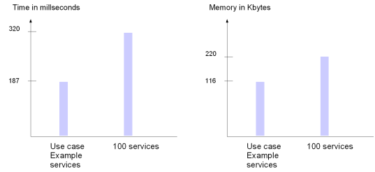
Figure 14: Time and memory consumption for syntactic service matching
