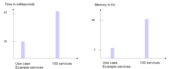
Figure 16: Time and memory consumption for QoS degree computing
