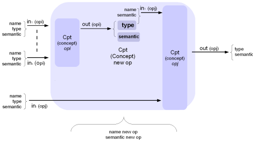
Figure 7: Service composition type or semantic compatibility
