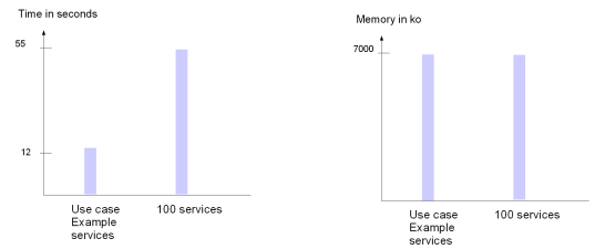
Figure 15: Time execution for semantic service matching
