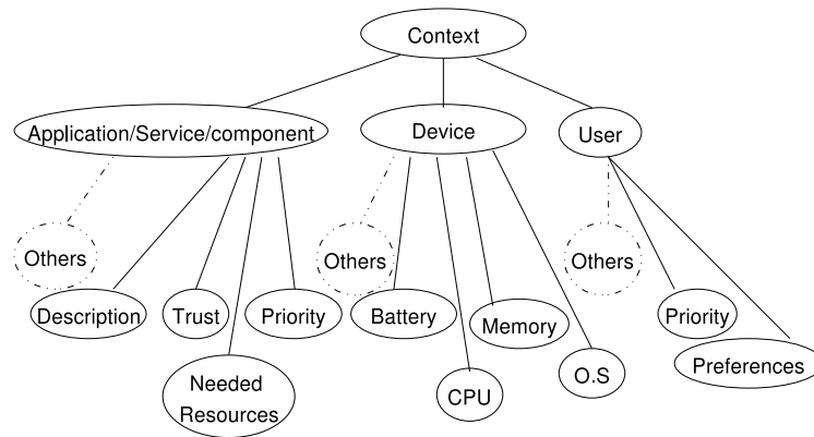
Fig. 2. Context Model
