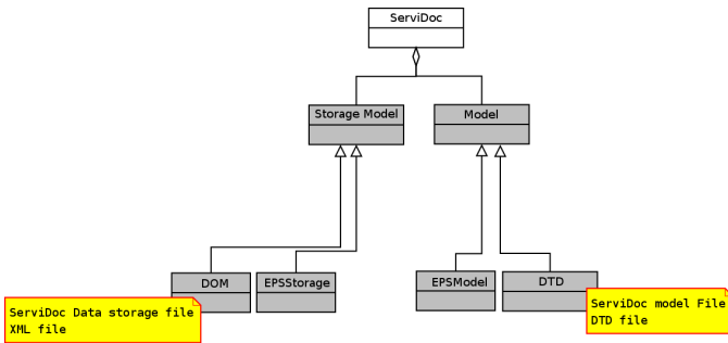
Fig. 4. ServiDoc Architecture
