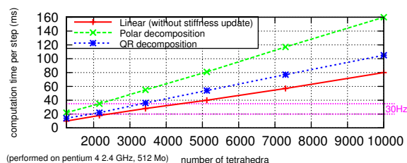
Figure 7: Computation time per time step against number of tetrahedra (with stiffness update, without assembly).
