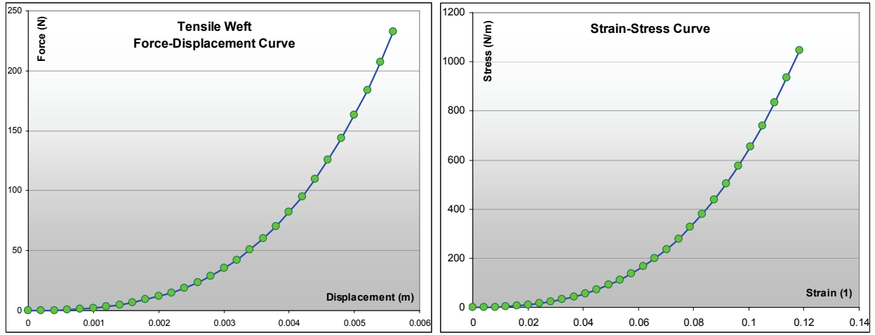
Figure 14: Converting a tensile force-deformation curve (left) in into a strain-stress curve (right) using the Kawabata standard sample size ( l_u = 0.05\text{m} , l_v = 0.2\text{m} ).
