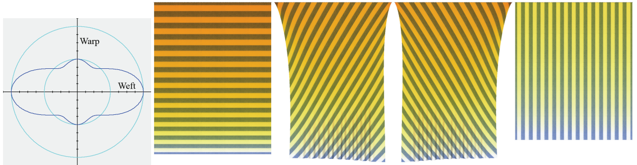
Figure 4: A large square piece of cloth cut along various fiber directions, hanging attached at one edge. The material is linear anisotropic (3), with 2 E_{uu,uu} = 1 E_{vv,vv} = 8 E_{uv,uv} (radial elongation stiffness diagram far left). This represents typical anisotropy of cloth materials, which usually have a much lower shear/elongation stiffness ratio than isotropic materials. Strips show weft fiber direction. Colorscale shows average tensile strain.
