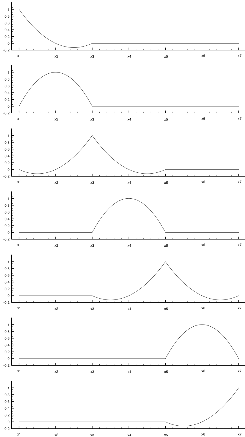
Figure 7: Example of one-dimensional quadratic Ritz functions.
