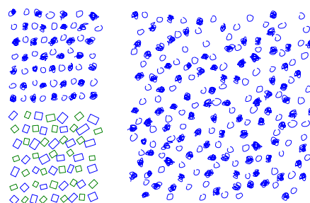
Figure 8: This example illustrates the main limitation of the Strauss model. Since it only accounts to second order interactions, it cannot reproduce well strongly regular arrangements such as this reference whose elements are pasted onto on a rectangular lattice. More sophisticated models that uses higher order interactions could be investigated to push back this limitation.
