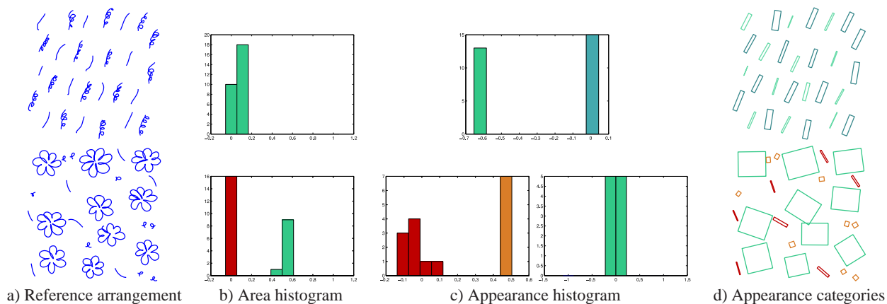
Figure 3: Categorization process Given a reference arrangement (a), the modes of the area histogram are first detected (b). In this example, one mode is found for the top row, while two are identified for the bottom row corresponding to the small and large elements. For each resulting area category, modes of the appearance histogram are then computed (c). Here, two modes are detected for the first row, the most discriminative feature being the number of crossings. The bottom row displays the appearance histogram of small elements where two MM-modes appear (blue and green modes). Only one MM-mode has been detected on the appearance histogram (red mode) for the larger element set. The resulting categories are finally shown with corresponding colors (d).
