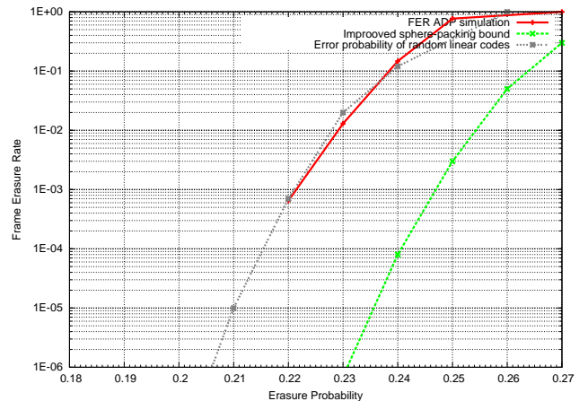
Fig. 6. Performance of the RS Code (255,191) over the BEC compared to the Sphere Packing lower Bound and the exact decoding error Probability of random binary linear block under ML decoding for N = 2040 and R = 0.75 .
