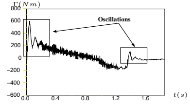
Fig. 6. Measured torque
