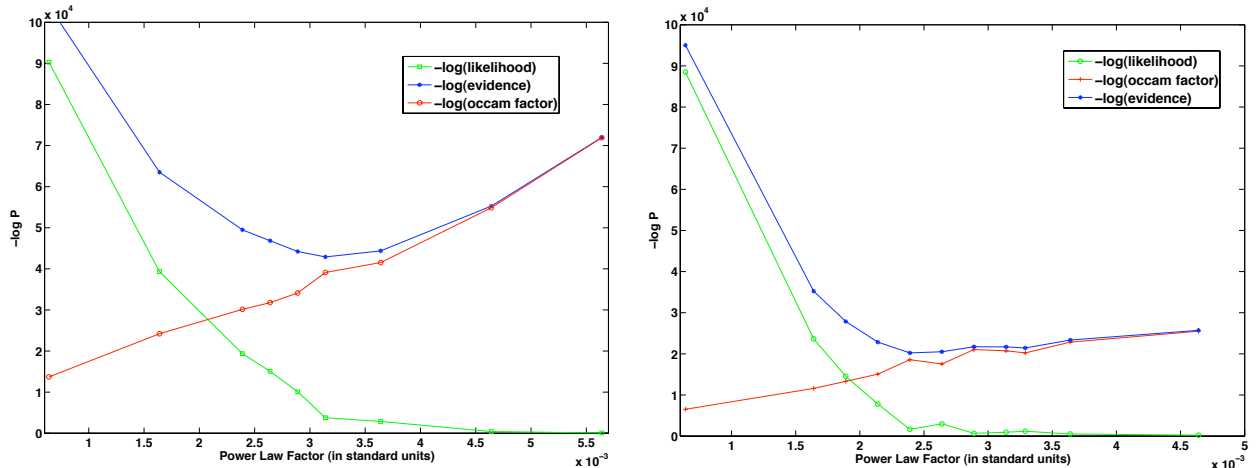
Figure 8: Evidence maximization w.r.t energy flux . Minus log of evidence (blue), likelihood (green) and Occam factor (red) v.s. power law factor \beta (i.e. energy flux \epsilon ) for horizontal winds at low ( left ) and at intermediate ( right ) altitude
