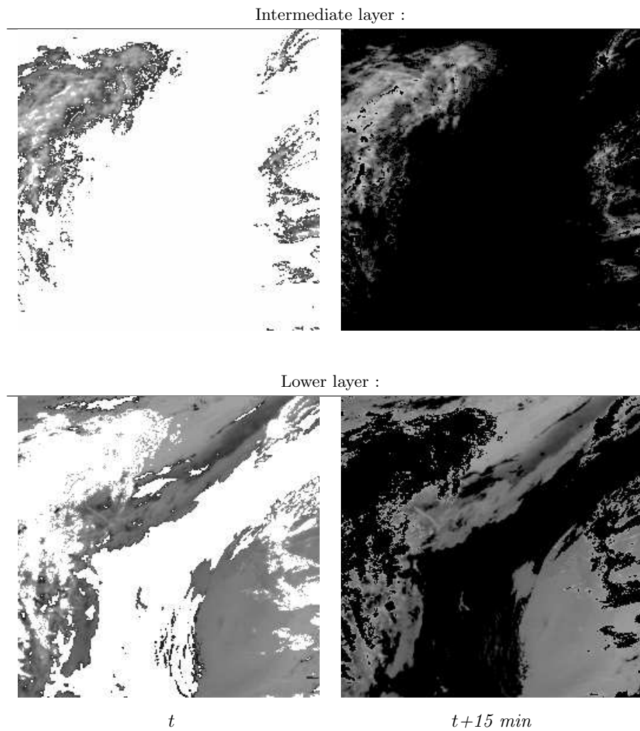
Figure 7: Input meteorological images. Sparse pressure difference maps of layers at intermediate (above) and low (below) altitude. White pixels of image at time t and black pixels at time t + 15 minutes are areas with no observations. The images characterize the layers evolution in a time interval of 15 minutes.
