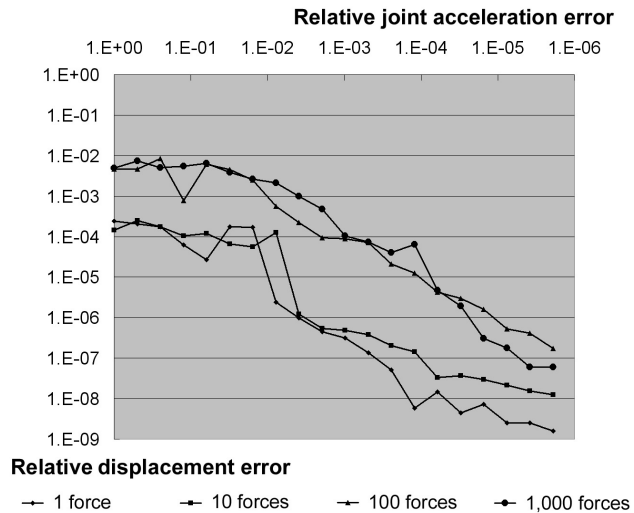
Figure 9: Influence of the relative joint acceleration error on the relative displacement error. As the precision enforced on the computation of the joint acceleration increases, the precision in the final configuration of the linkage expressed in the world frame increases as well.
