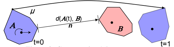
Figure 3: Conservative Advancement.
