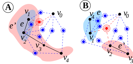
Fig. 8. When \text{card}(V_0) = 5 , \text{card}(\mathcal{E}) = 8 and two hyperedges, e and e' , of \mathcal{E} contains several vertices of V_0 . The paths corresponding to potential insertions of elements of V_2 and V_3 are drawn in dashed lines. In this figure, the positions of the vertices of V_2 and V_3 w.r.t. e and e' are not significant.
