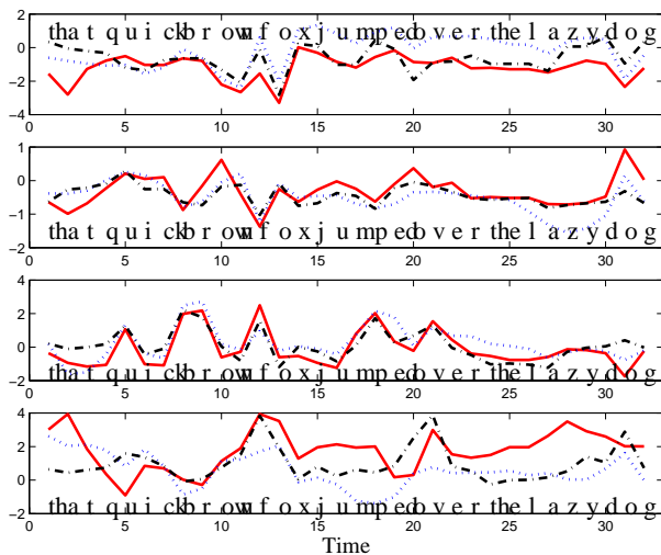
Figure 6: Results for three subject, time-aligned on the phonemes of the same uttered sentence. Subject 1: RED, Subject 2: BLUE, and Subject 3: BLACK.
