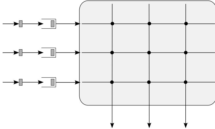
Figure 4: Input Queueing architecture
