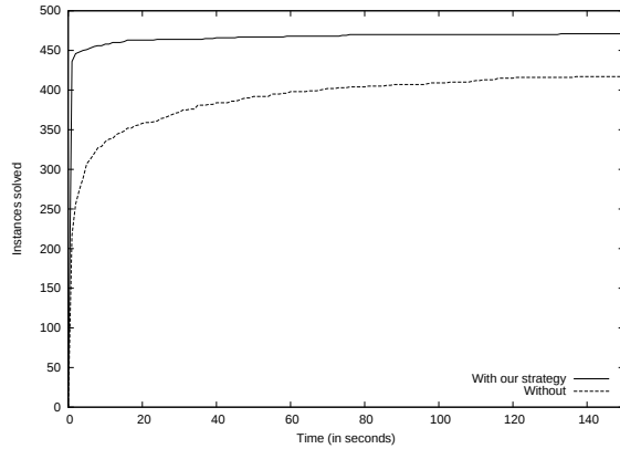
Figure 8. Number of instances of the OCC solved within a short time limit : comparison of the cutting-plane algorithm efficiency when using (or not) our strategy.
