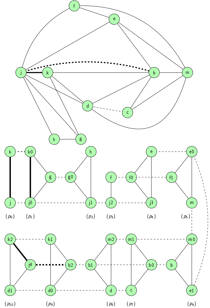
Figure 2. A small program and its interference graph (top). Full edges are interference edges. Affinity edges are dashed edges. The same program after extreme live-range splitting and its split interference graph (bottom). The weights of affinity edges are omitted in the Figure. The program points (p_0) \dots (p_{10}) of both programs are shown in the Figure.
