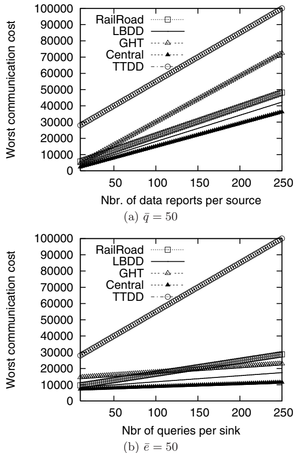
Figure 4: Worst-case Communication cost ( m = 5 sinks, n = 10 sources).
