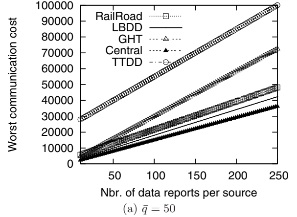
Figure 4: Worst-case Communication cost ( m = 5 sinks, n = 10 sources).
