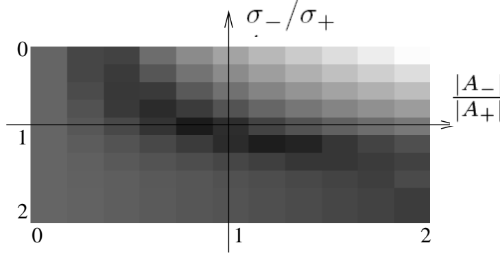
Figure 3: Representation of |\bar{\mathbf{W}}| magnitude variations for Mexican-hat profiles. Here the 2D scalar map size is 100 \times 100 and \sigma_+ = 10 , while A_+ = 1/20 , for magnitudes between 0 (black) and 1 (white). Results are obtained in less than 5 iterations of the power-method. We observe the non trivial increase and decrease of the magnitude depending on the inhibitory/excitatory gain and width ratios: It increases with \sigma_-/\sigma_+ and decreases with |A_-|/|A_+| when \sigma_- < \sigma_+ and |A_-| < |A_+| which corresponds to the intuition that inhibition “balances” excitation. A dual effect is observed when \sigma_- > \sigma_+ and |A_-| > |A_+| : Inhibition, when not thresholded by the rectification mechanism, also induces high magnitudes, thus instabilities. In other conditions the magnitude is not monotonic.
