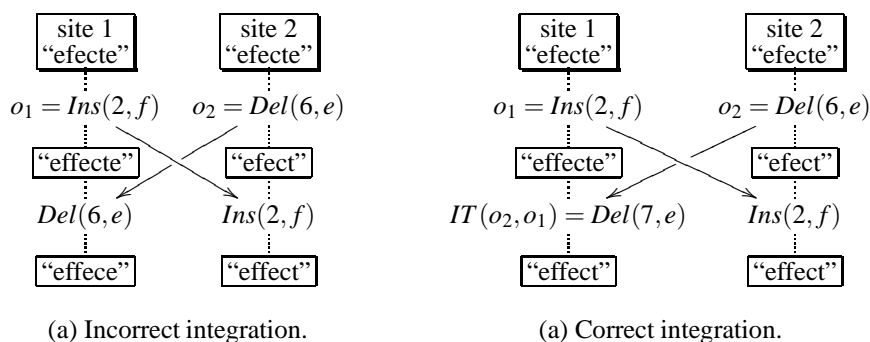
Figure 1: Serialization of concurrent cooperative operations
