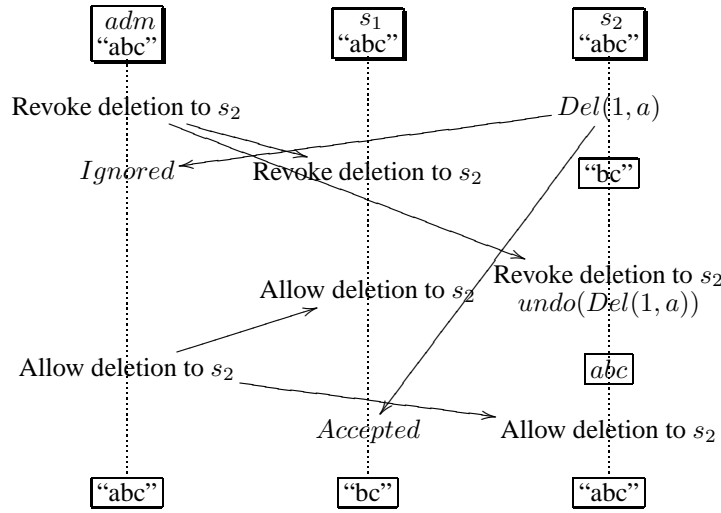
Figure 3: Necessity of admin Log.
