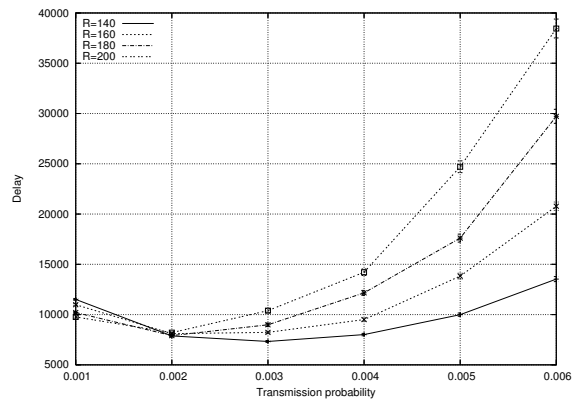
Fig. 7. Shortest path routing algorithm: end-to-end delay versus p for various transmission ranges.
